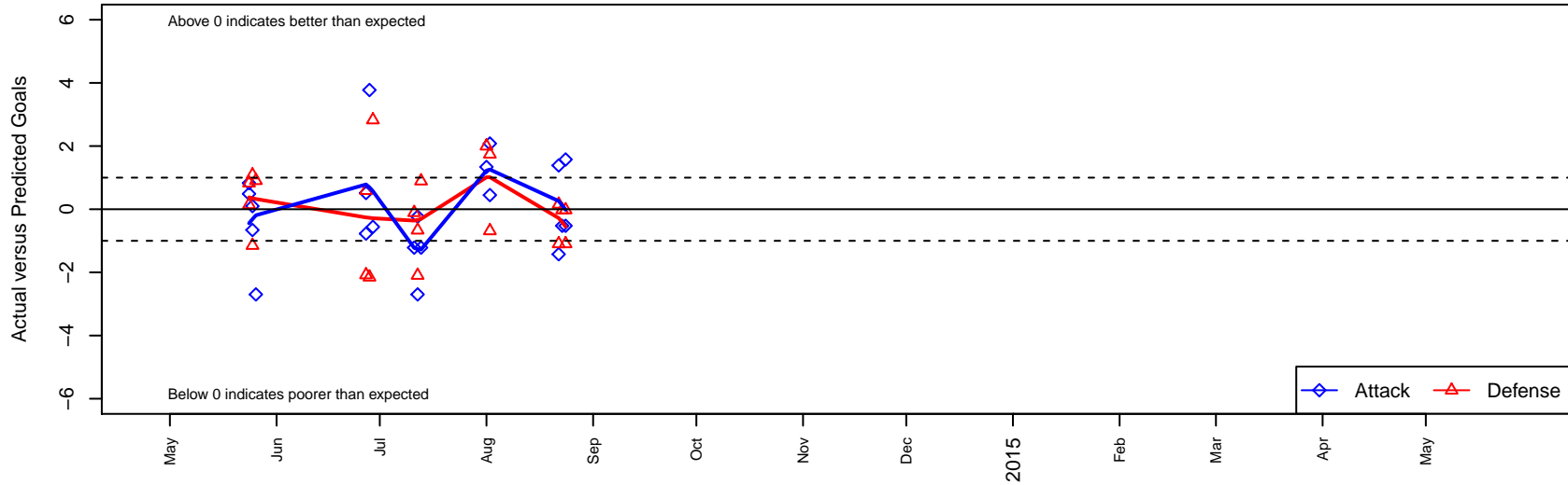
Albany FC Heat B01 Dots are actual minus expected GF (blue circles) and GA (red triangles). Blue line is smoothed change in attack strength. Red is smoothed change in defense strength.
